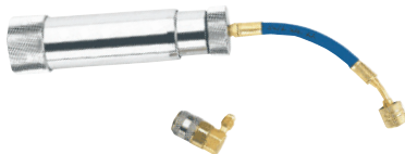
FJC2732 A/C Oil and Dye Injector R12 and R134A 2 oz.
